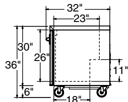
MBUR/MBUF48A ELEVATION VIEW
