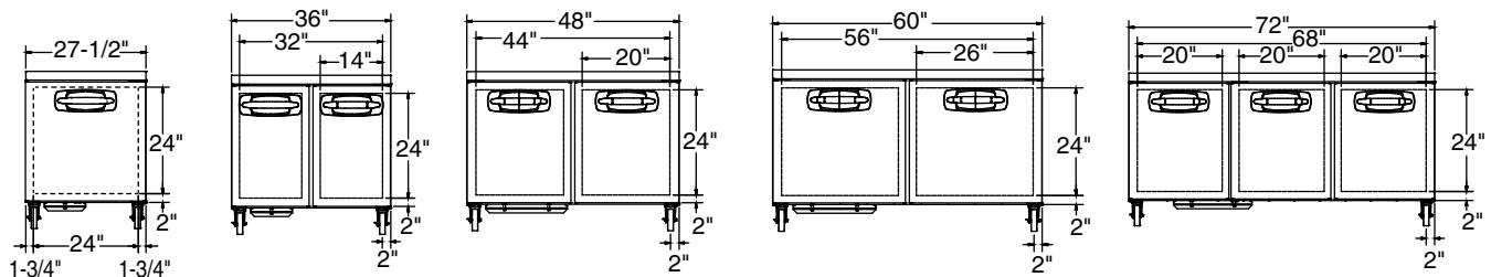
MBUR/MBUF27A ELEVATION VIEW
