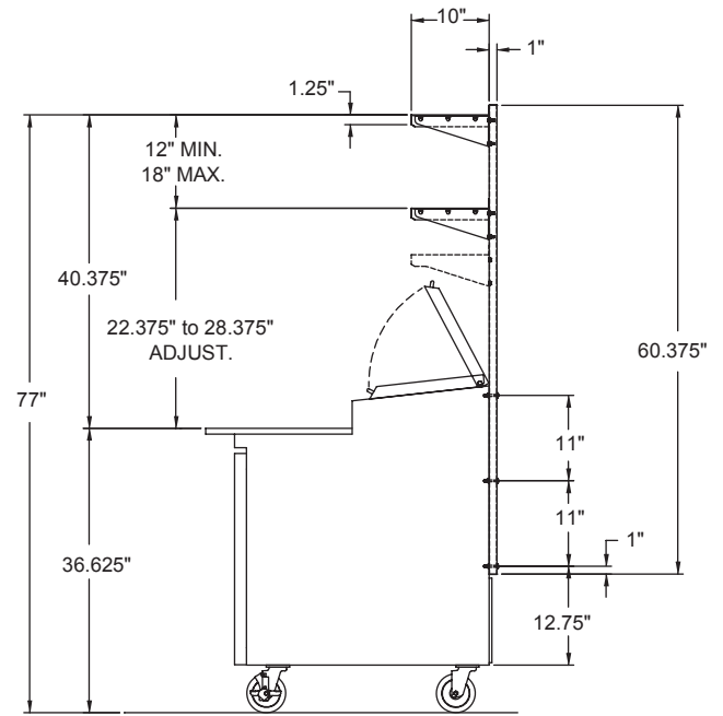
SECTION - 1
