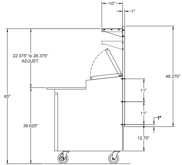
SECTION - 1
