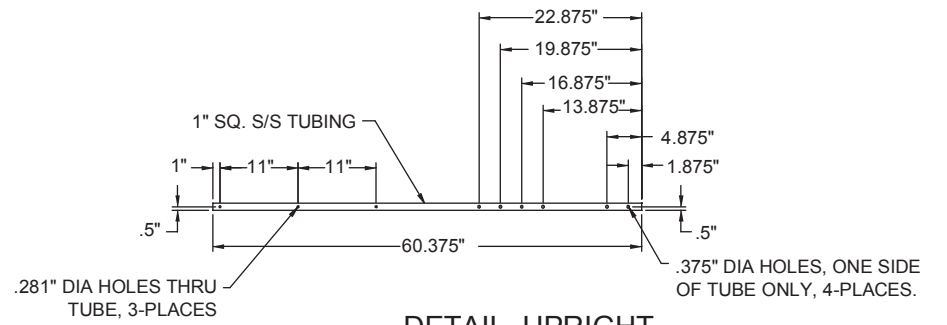
DETAIL, UPRIGHT
