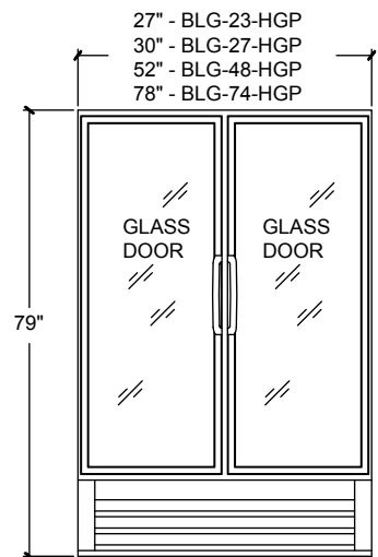
ELEVATION VIEW
