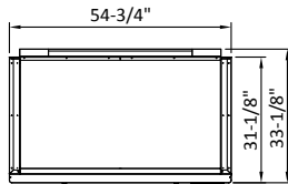
MBTR23-S/MBTF23-S PLAN VIEW
