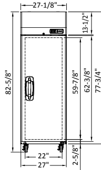
MBTR23-S/MBTF23-S ELEVATION VIEW
