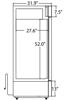
ALL MODELS SIDE VIEW
