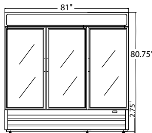
MBRGM72HB/MBFGM72HB ELEVATION VIEW
