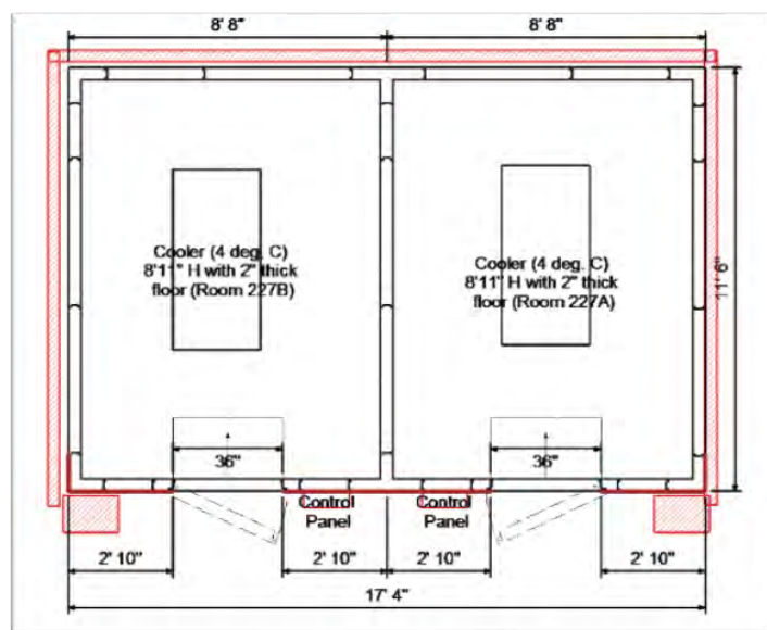
Construction Diagram
